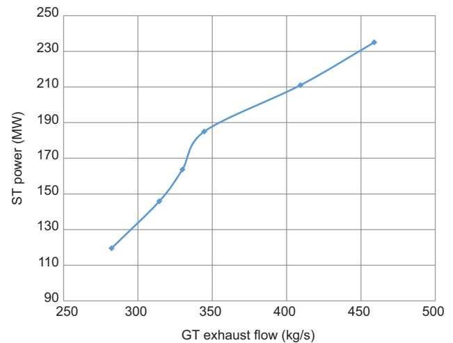
Fig. 11. Steam turbine power generation during part-load operation versus gas turbine exhaust flow.
